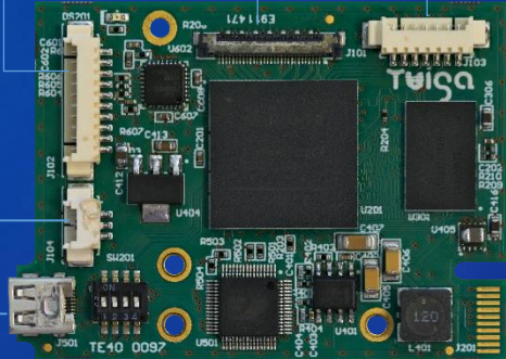
J101 Tamron LVDS Camera Input
